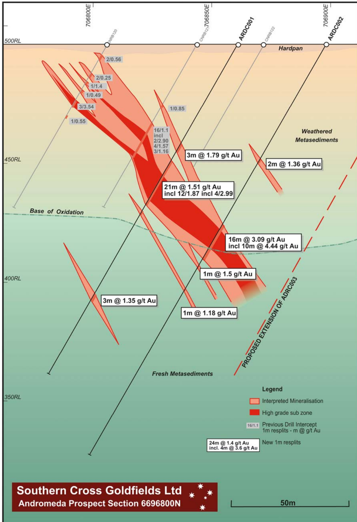
Figure 1 – Andromeda Cross Section – 6800N
